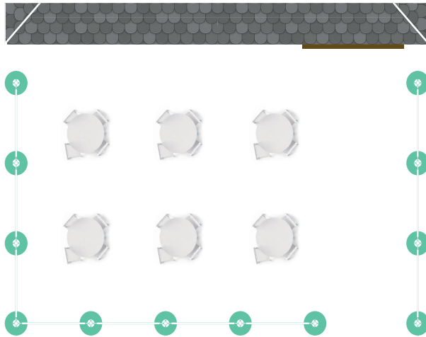
1. 12 posts/bases & 10 cross rails.
